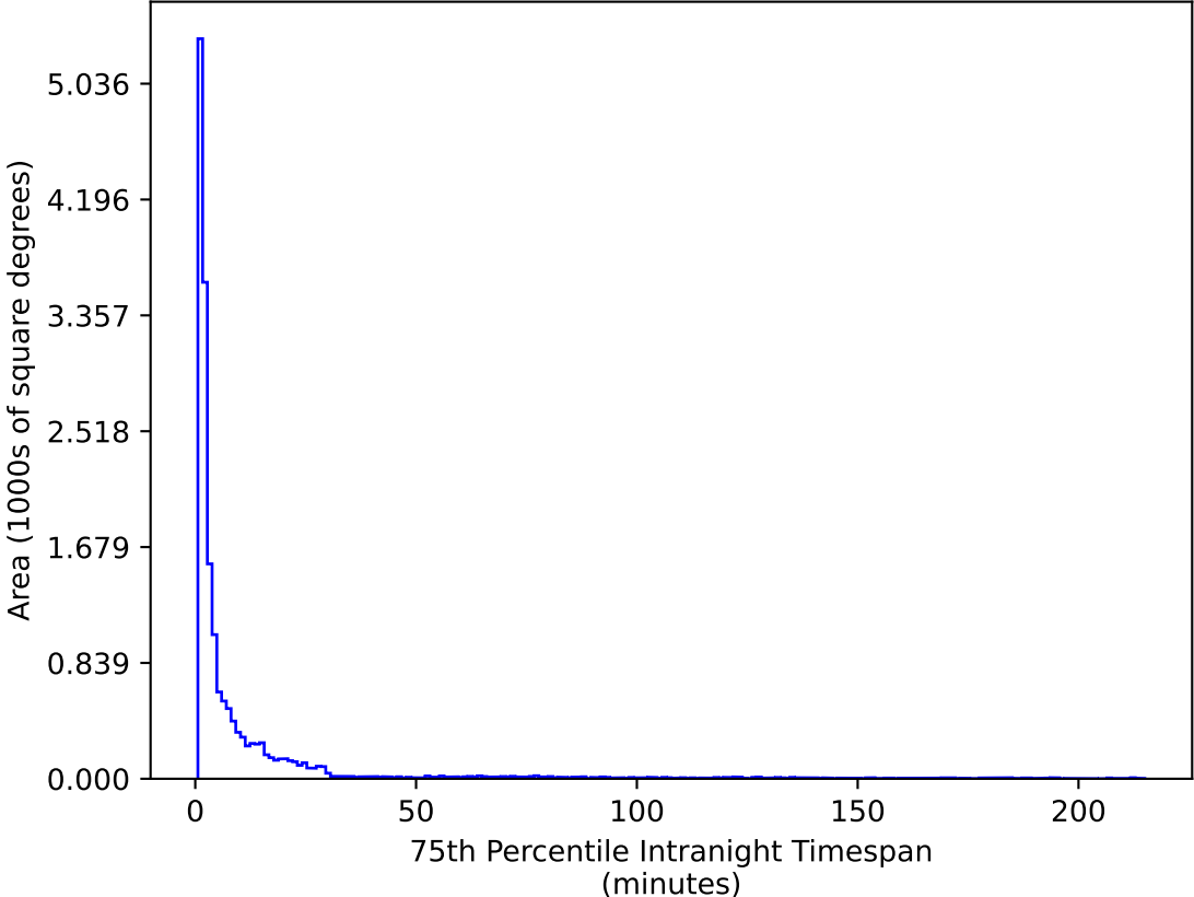
too_elab_r64_d2_gz_v3.4_10yrs WFD u band: 75th Percentile Intranight Timespan
