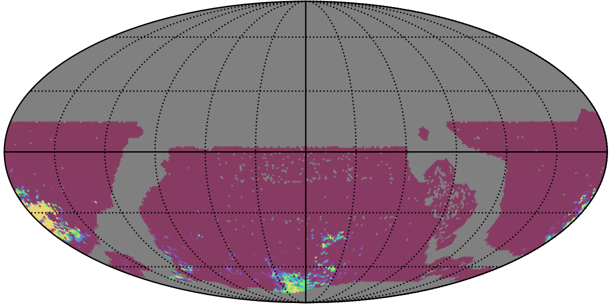
too_elab_r64_d2_gz_v3.4_10yrs WFD gr bands: 75th Percentile Intranight Timespan
