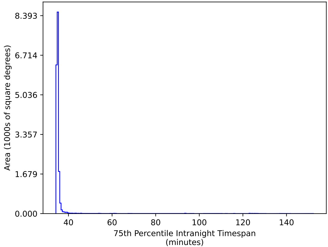
too_elab_r64_d2_gz_v3.4_10yrs WFD gr bands: 75th Percentile Intranight Timespan
