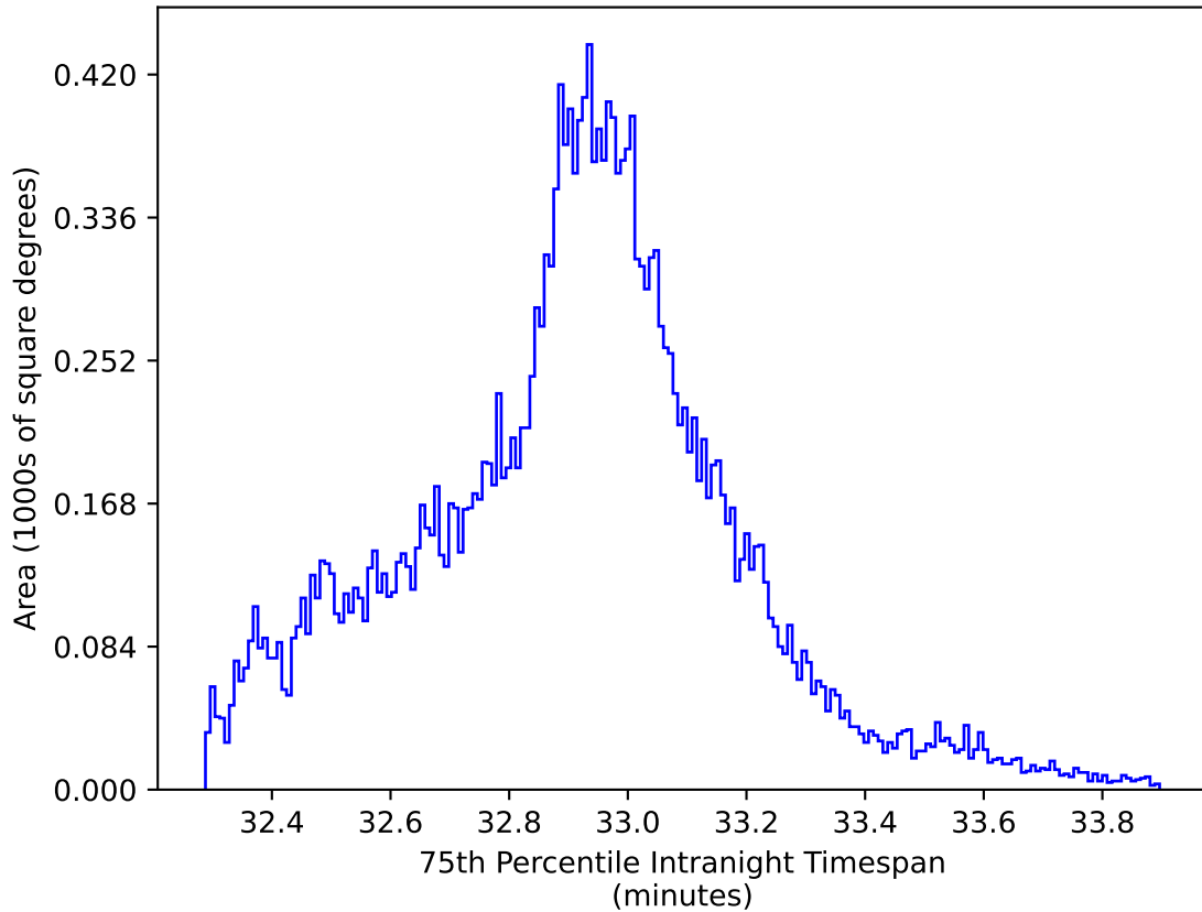
too_elab_r64_d2_gz_v3.4_10yrs All sky y band: 75th Percentile Intranight Timespan
