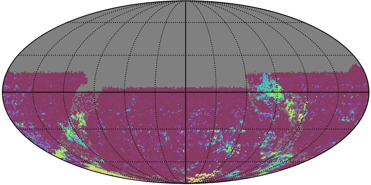
too_elab_r64_d2_gz_v3.4_10yrs All sky u band: 75th Percentile Intranight Timespan
