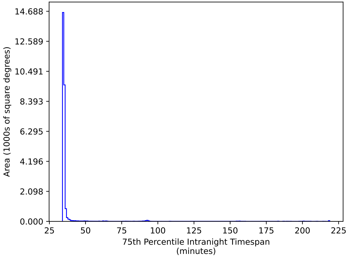
too_elab_r64_d2_gz_v3.4_10yrs All sky ri bands: 75th Percentile Intranight Timespan
