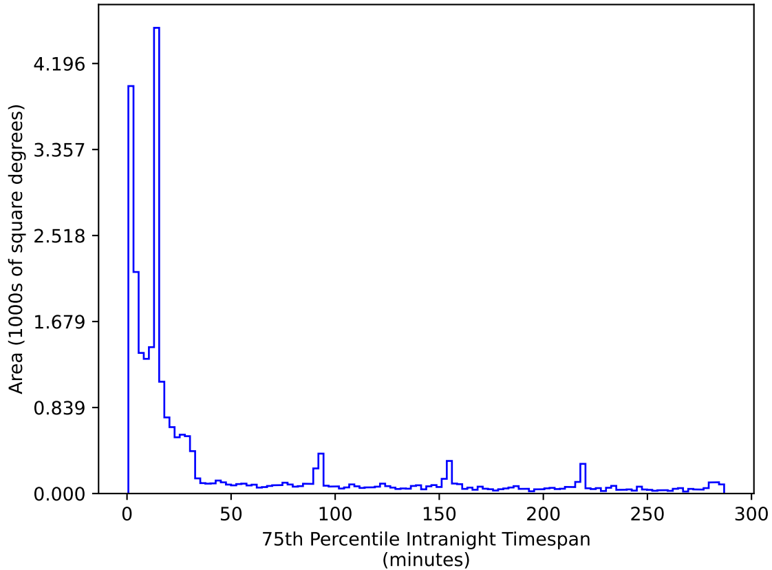
too_elab_r64_d2_gz_v3.4_10yrs All sky r band: 75th Percentile Intranight Timespan
