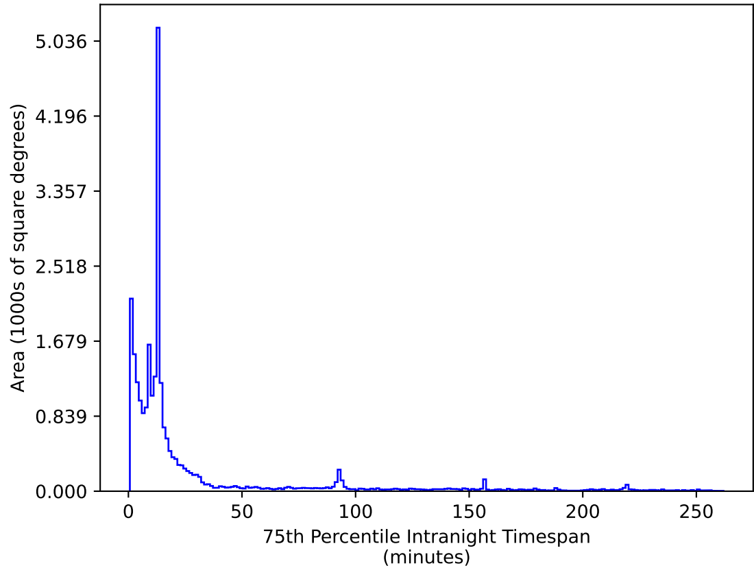
too_elab_r64_d2_gz_v3.4_10yrs All sky i band: 75th Percentile Intranight Timespan
