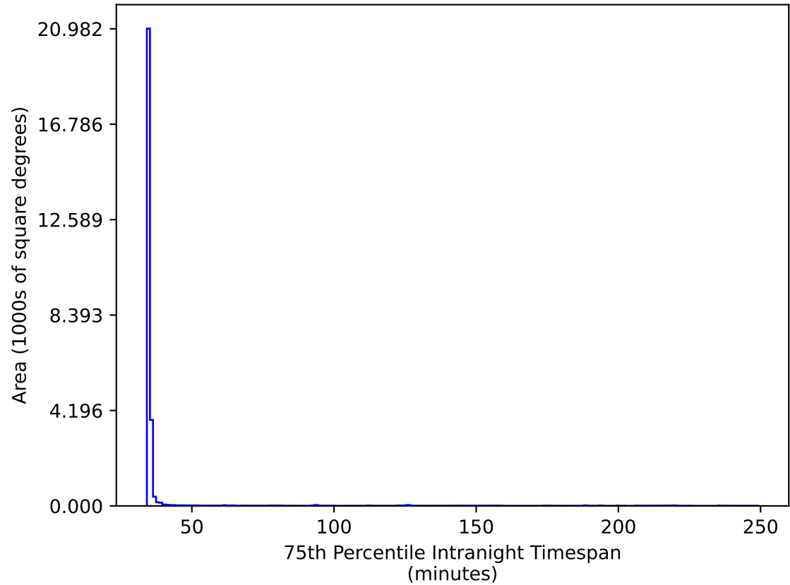
too_elab_r64_d2_gz_v3.4_10yrs All sky gr bands: 75th Percentile Intranight Timespan
