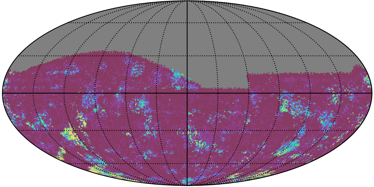
too_elab_r64_d2_gz_v3.4_10yrs All sky g band: 75th Percentile Intranight Timespan
