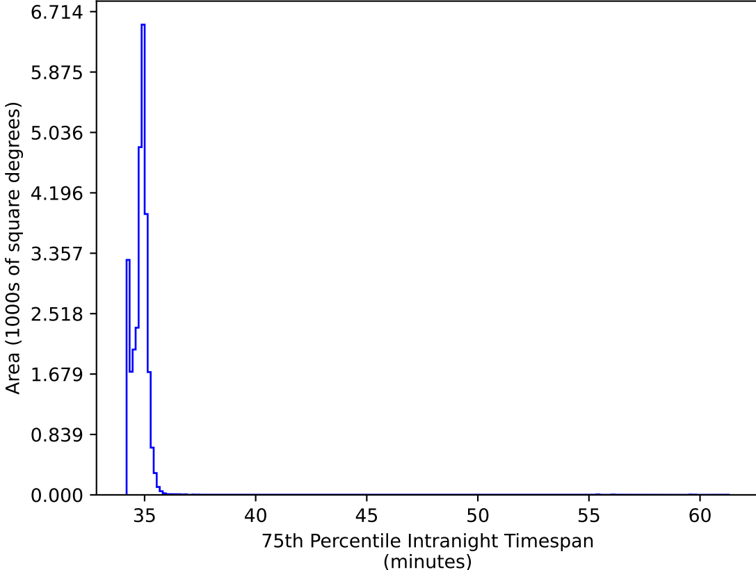
too_elab_r64_d2_gz_v3.4_10yrs All sky all bands: 75th Percentile Intranight Timespan
