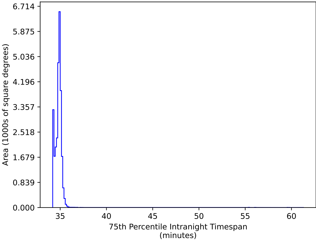
too_elab_r64_d2_gz_v3.4_10yrs All sky: 75th Percentile Intranight Timespan
