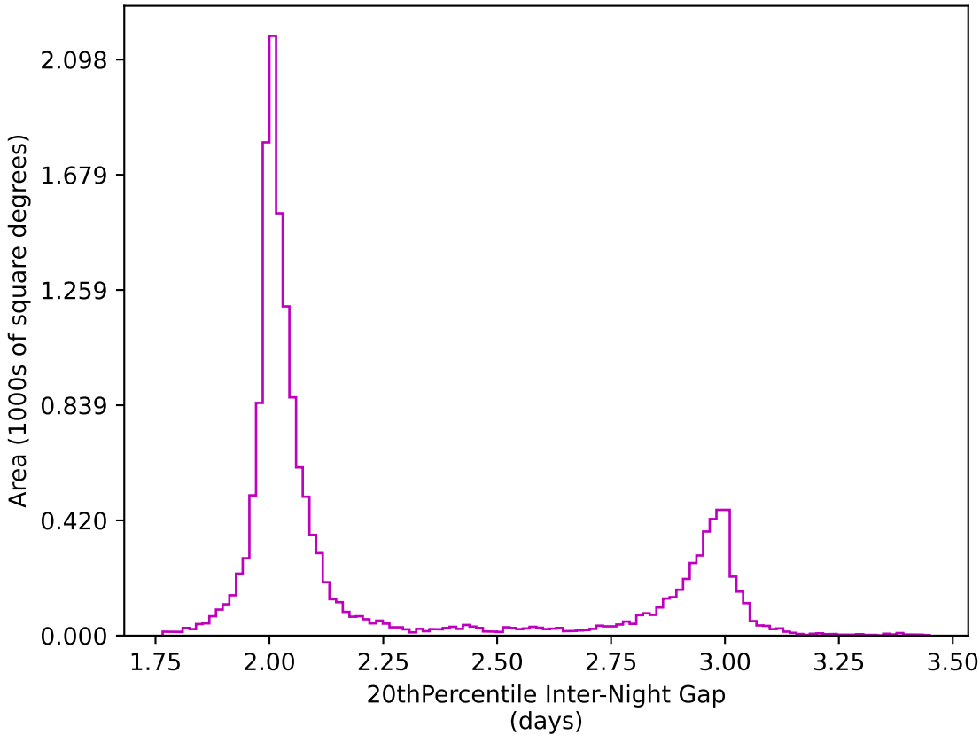
too_elab_r64_d2_gz_v3.4_10yrs WFD z band: 20thPercentile Inter-Night Gap
