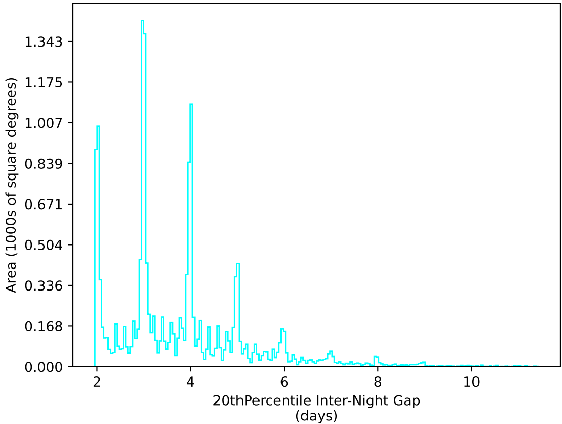
too_elab_r64_d2_gz_v3.4_10yrs WFD u band: 20thPercentile Inter-Night Gap
