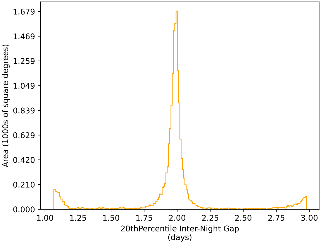
too_elab_r64_d2_gz_v3.4_10yrs WFD r band: 20thPercentile Inter-Night Gap
