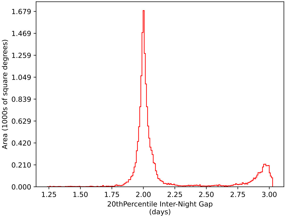
too_elab_r64_d2_gz_v3.4_10yrs WFD i band: 20thPercentile Inter-Night Gap
