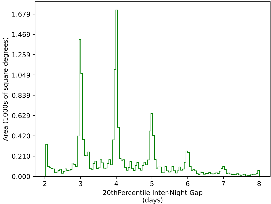
too_elab_r64_d2_gz_v3.4_10yrs WFD g band: 20thPercentile Inter-Night Gap
