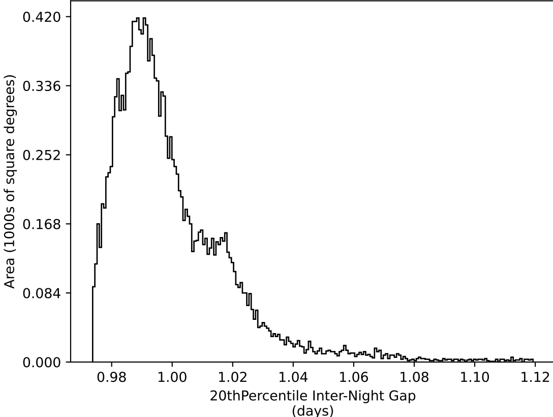
too_elab_r64_d2_gz_v3.4_10yrs WFD all bands: 20thPercentile Inter-Night Gap
