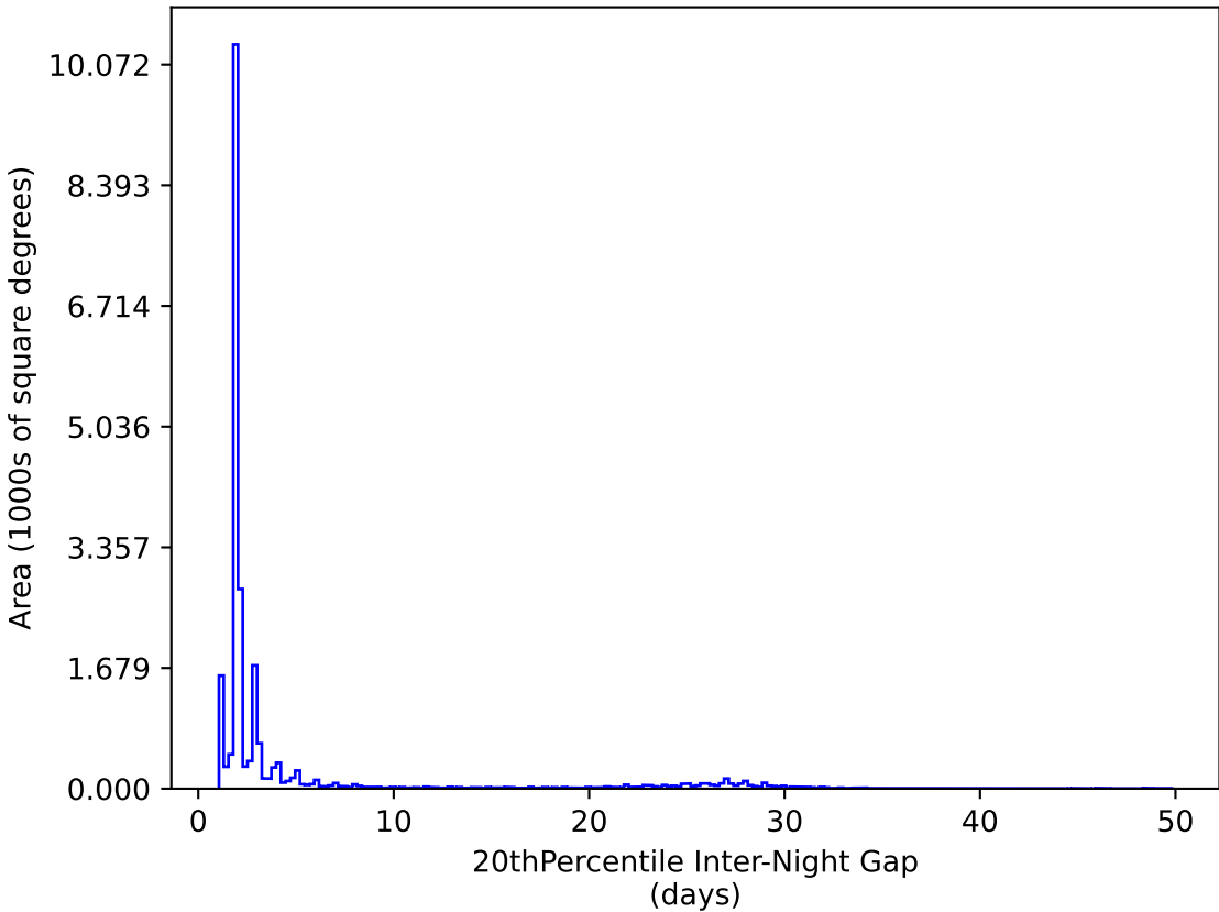
too_elab_r64_d2_gz_v3.4_10yrs All sky y band: 20thPercentile Inter-Night Gap
