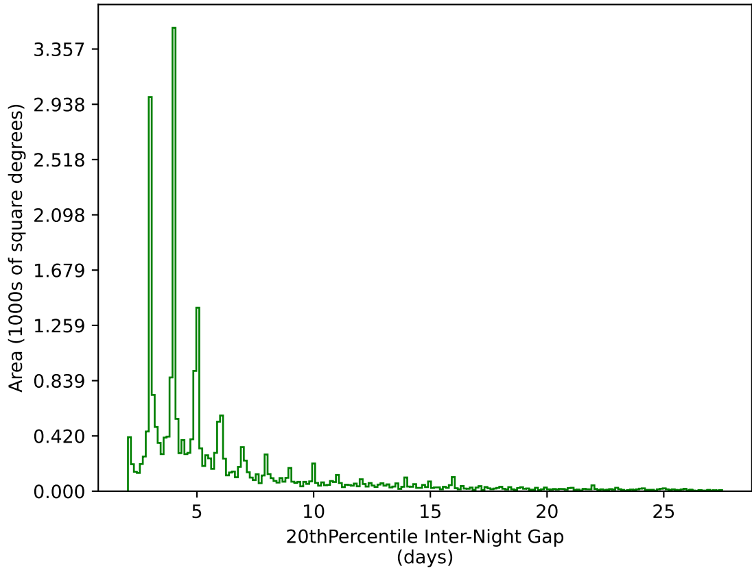
too_elab_r64_d2_gz_v3.4_10yrs All sky g band: 20thPercentile Inter-Night Gap
