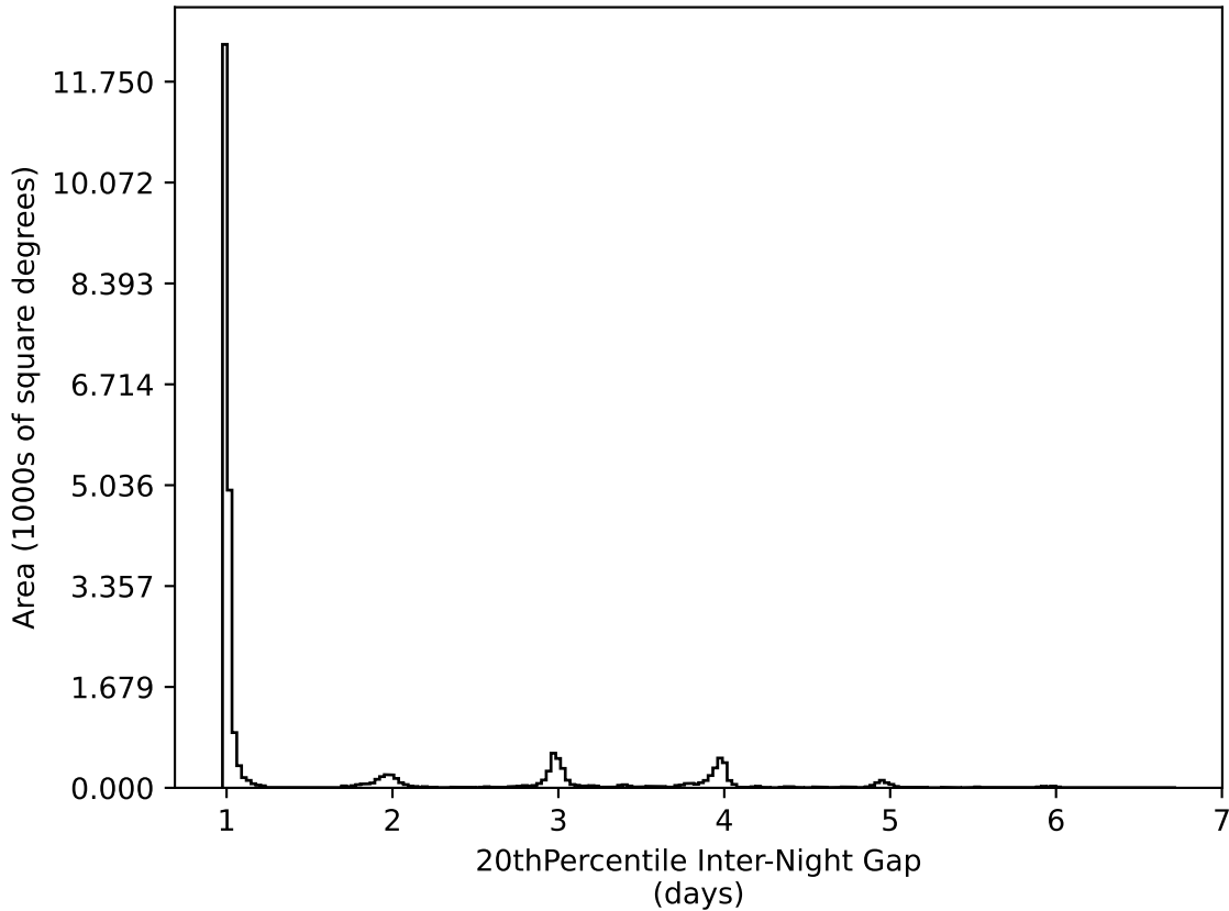
too_elab_r64_d2_gz_v3.4_10yrs All sky all bands: 20thPercentile Inter-Night Gap
