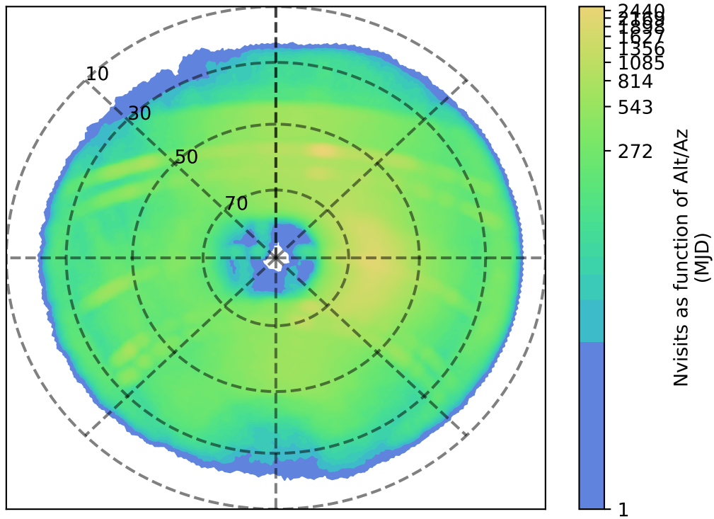
too_elab_r64_d2_gz_v3.4_10yrs z: Nvisits as function of Alt/Az
