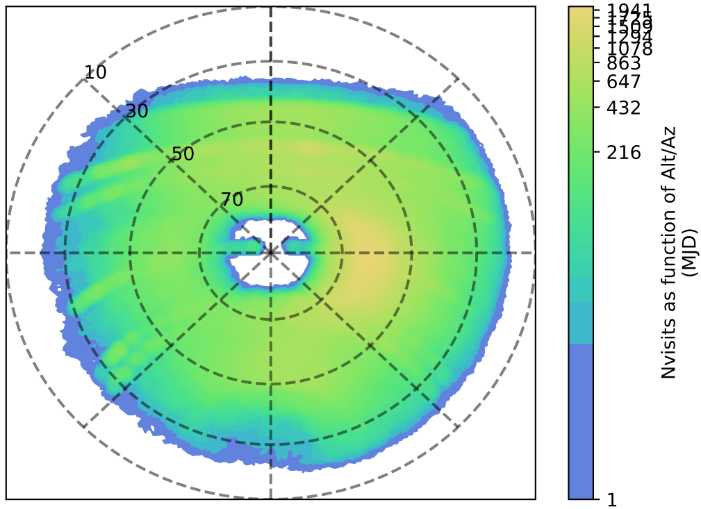
too_elab_r64_d2_gz_v3.4_10yrs y: Nvisits as function of Alt/Az
