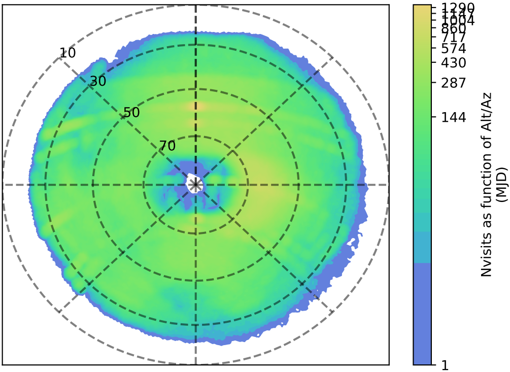
too_elab_r64_d2_gz_v3.4_10yrs g: Nvisits as function of Alt/Az
