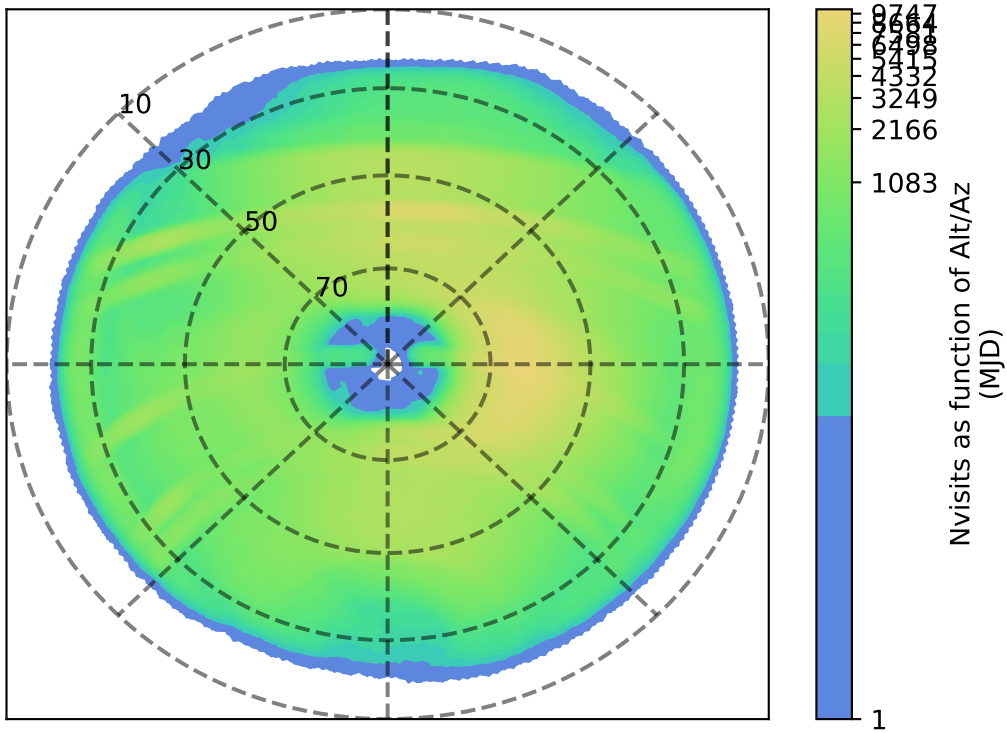
too_elab_r64_d2_gz_v3.4_10yrs : Nvisits as function of Alt/Az
