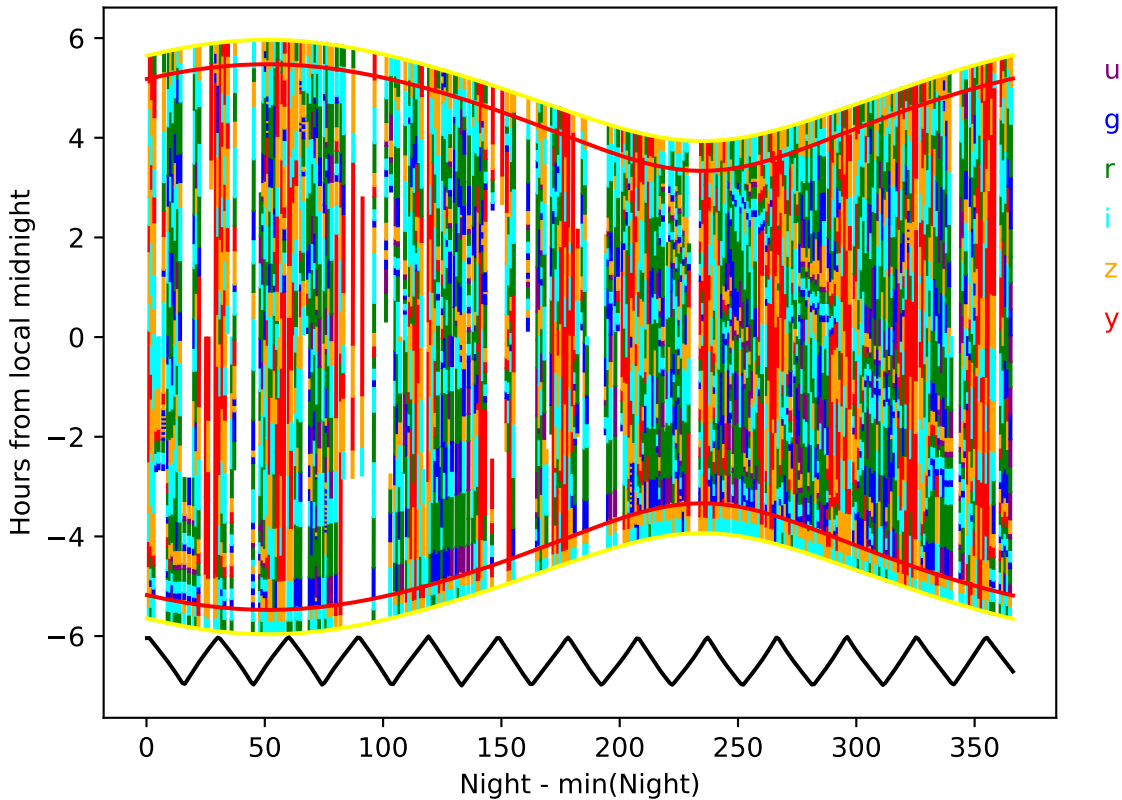
too_elab_r64_d2_gz_v3.4_10yrs year 1-2: Hourglass
