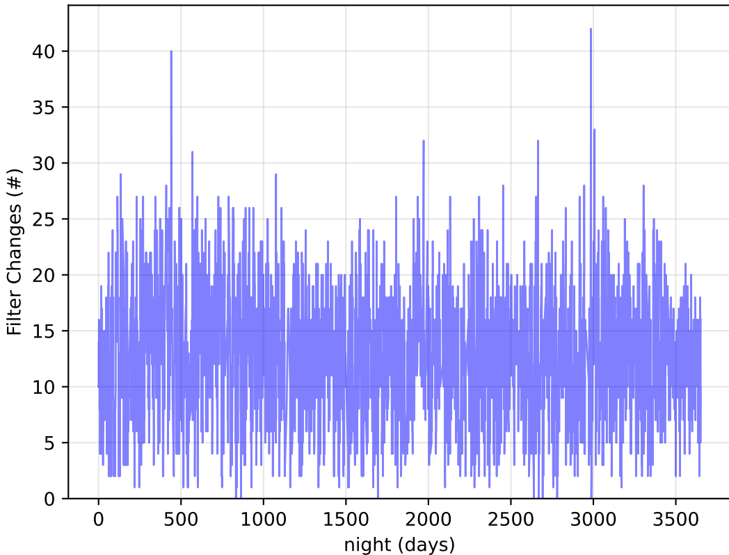
too_elab_r64_d2_gz_v3.4_10yrs : Filter Changes
