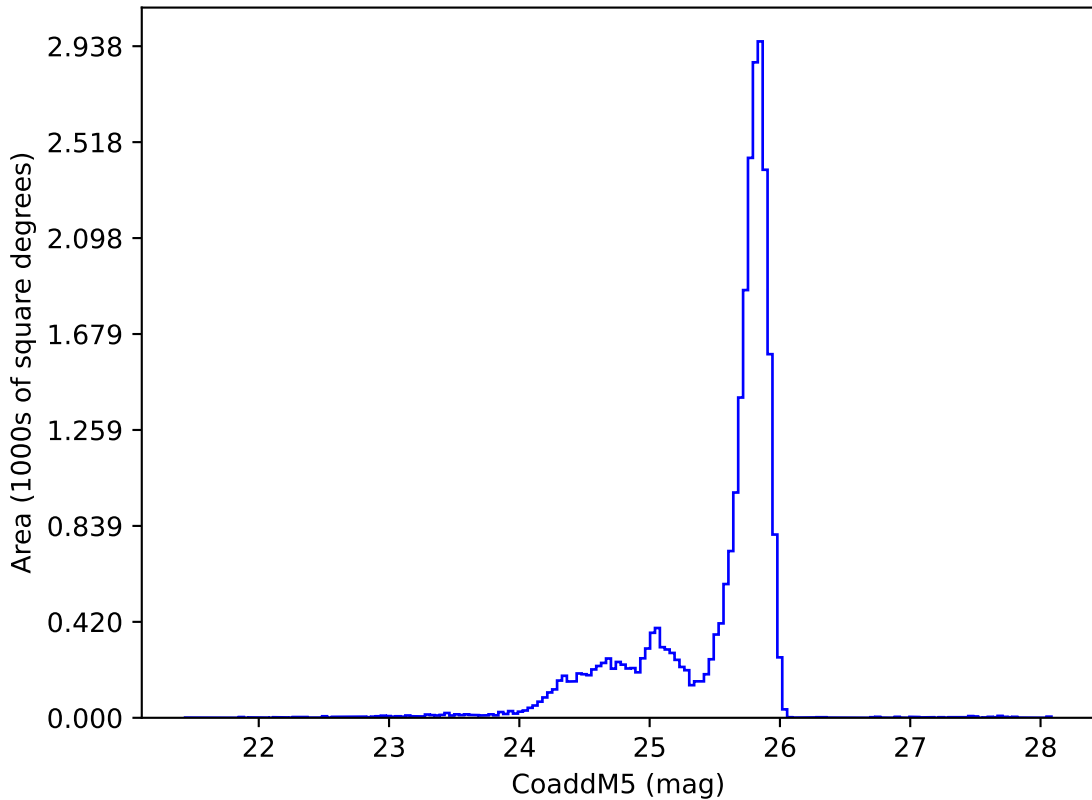
too_elab_r64_d2_gz_v3.4_10yrs z: CoaddM5
