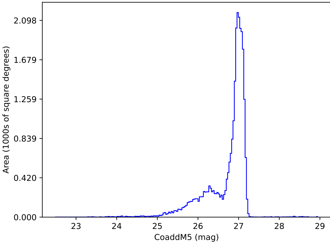
too_elab_r64_d2_gz_v3.4_10yrs r: CoaddM5
