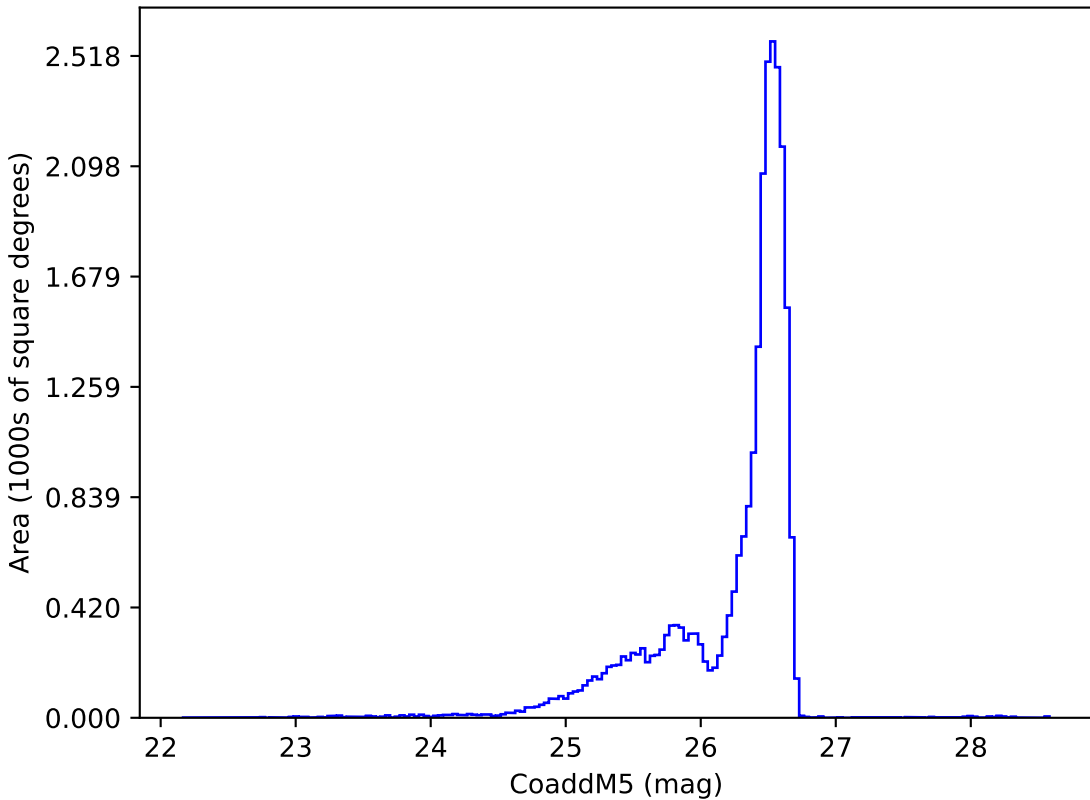
too_elab_r64_d2_gz_v3.4_10yrs i: CoaddM5
