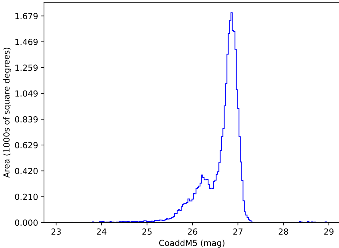
too_elab_r64_d2_gz_v3.4_10yrs g: CoaddM5
