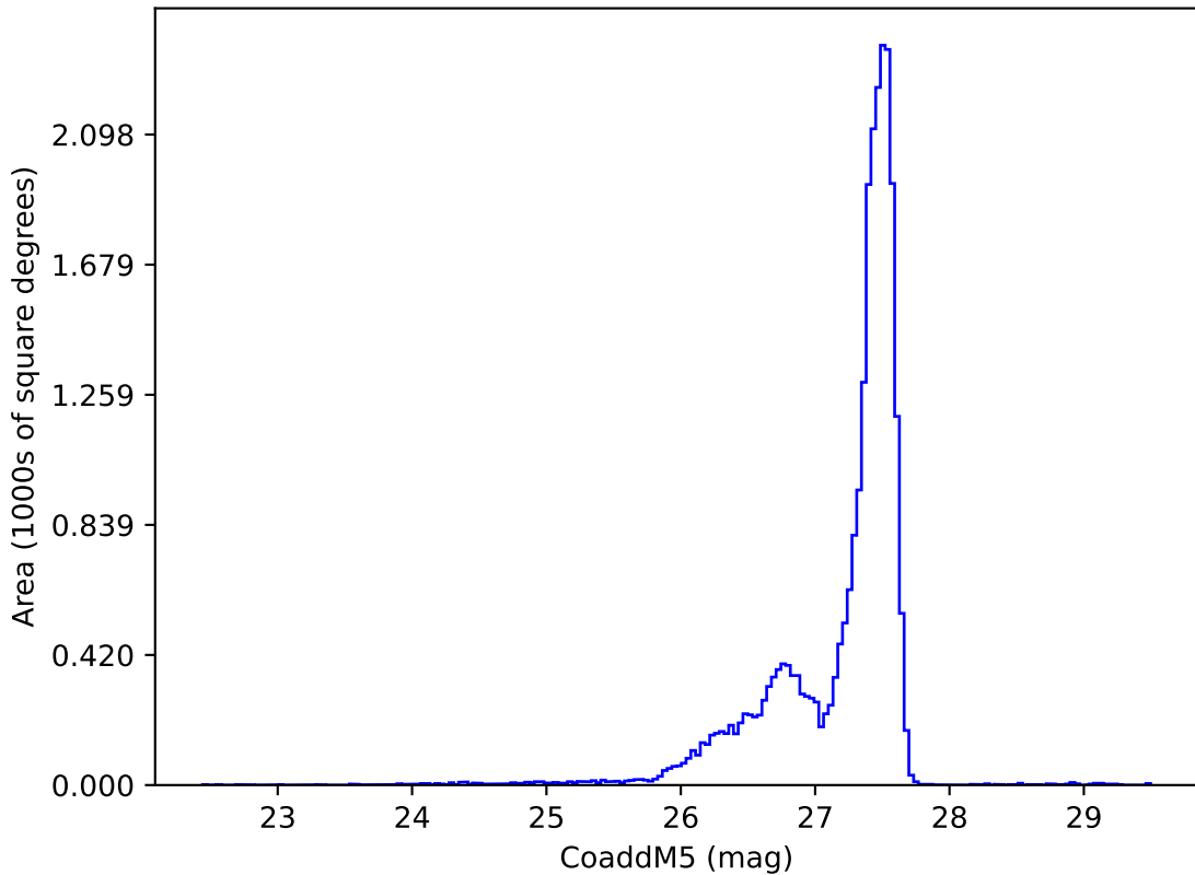
too_elab_r64_d2_gz_v3.4_10yrs : CoaddM5
