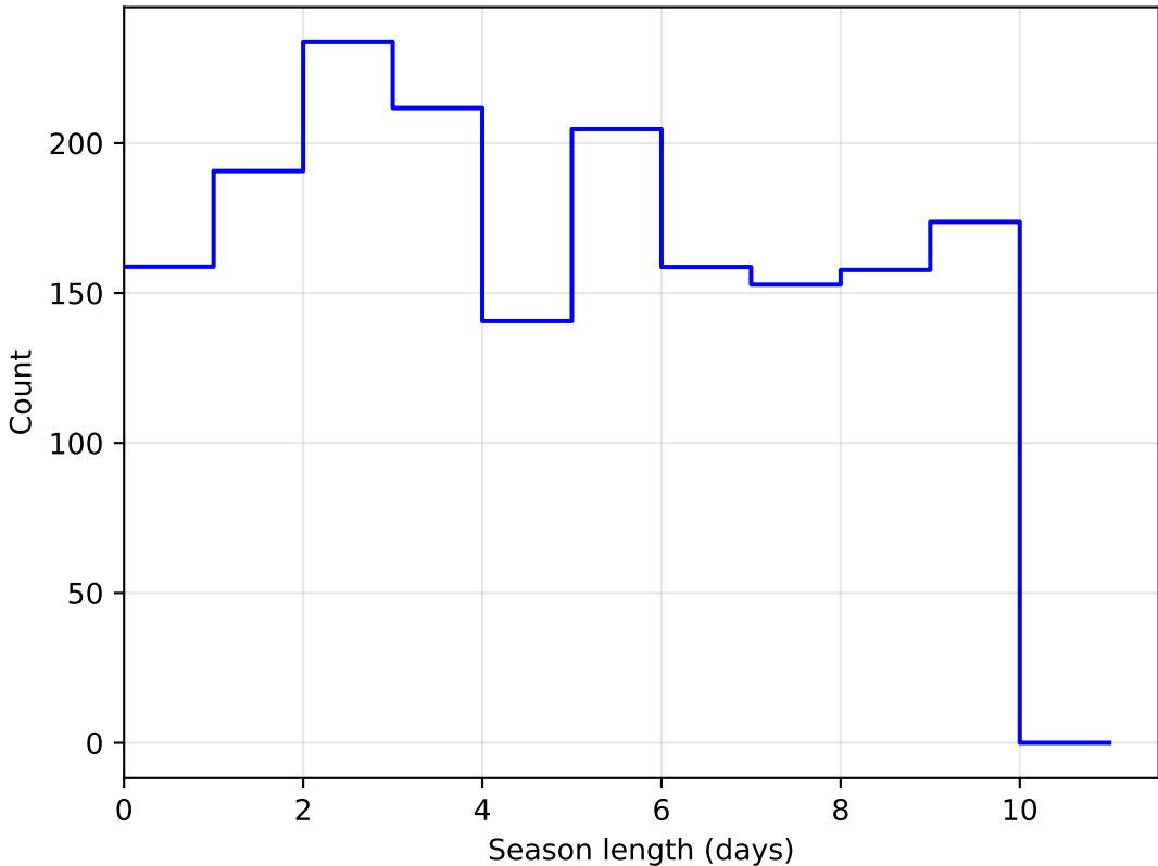
too_elab_r64_d2_gz_v3.4_10yrs DD:WFD all bands: SeasonLength
