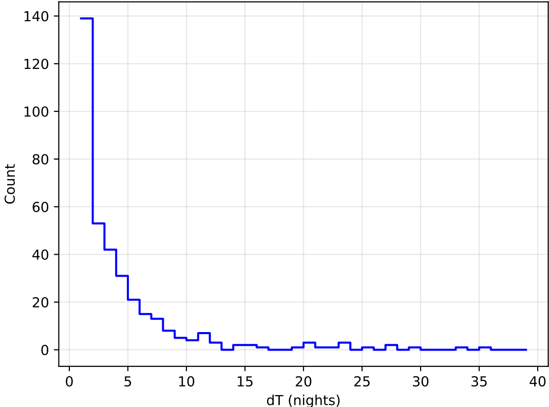
too_elab_r64_d2_gz_v3.4_10yrs all bands: DD:WFD Delta Nights Histogram
