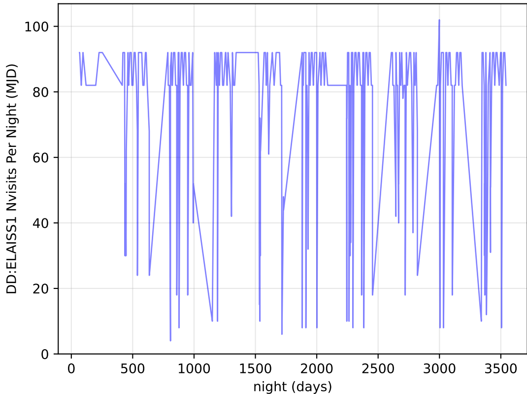
too_elab_r64_d2_gz_v3.4_10yrs all bands: DD:ELAISS1 Nvisits Per Night
