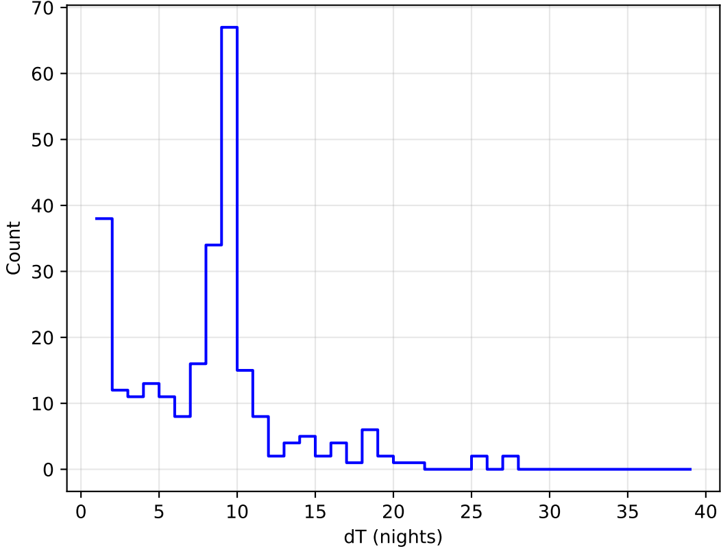
too_elab_r64_d2_gz_v3.4_10yrs all bands: DD:ELAISS1 Delta Nights Histogram
