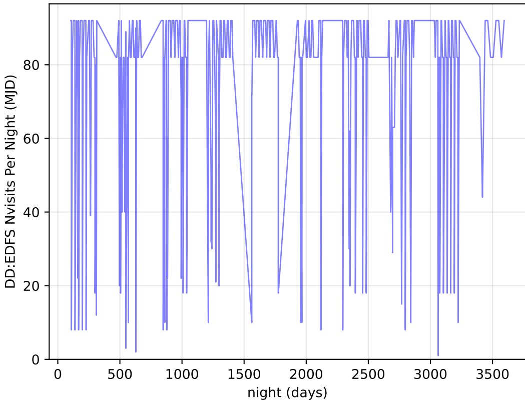
too_elab_r64_d2_gz_v3.4_10yrs all bands: DD:EDFS Nvisits Per Night
