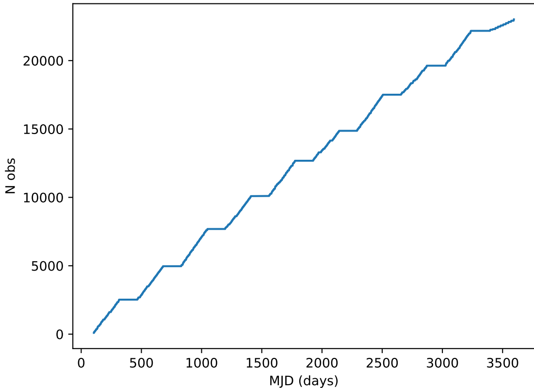
too_elab_r64_d2_gz_v3.4_10yrs all bands: DD:EDFS Cumulative NVisits
