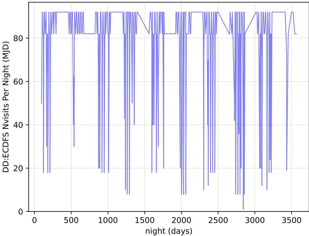
too_elab_r64_d2_gz_v3.4_10yrs all bands: DD:ECDFS Nvisits Per Night
