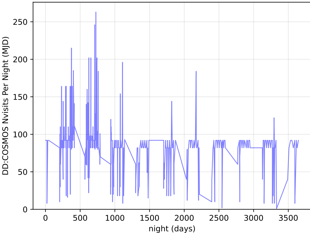
too_elab_r64_d2_gz_v3.4_10yrs all bands: DD: COSMOS Nvisits Per Night
