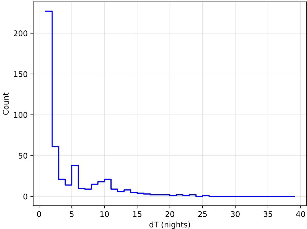
too_elab_r64_d2_gz_v3.4_10yrs all bands: DD: COSMOS Delta Nights Histogram
