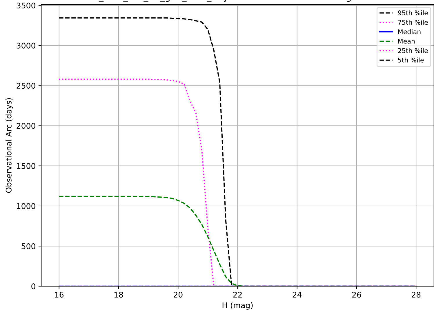
too_elab_r64_d2_griz_v3.4_10yrs: Observational Arc Length Vatira
