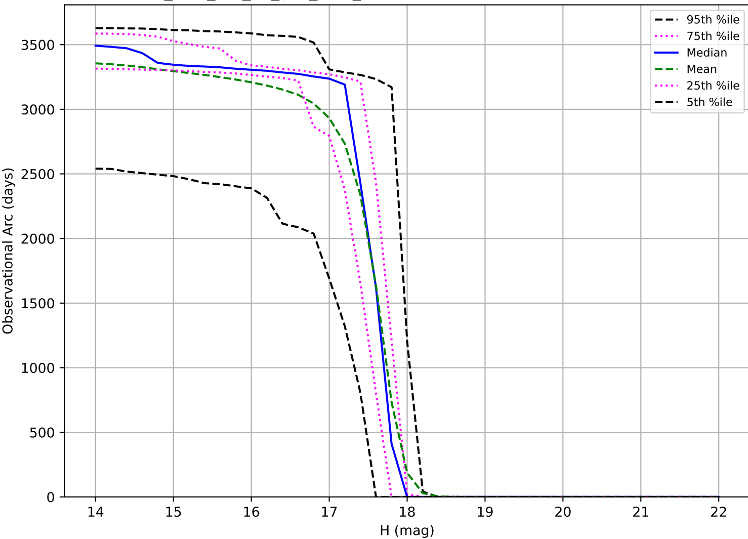
too_elab_r64_d2_griz_v3.4_10yrs: Observational Arc Length Trojan
