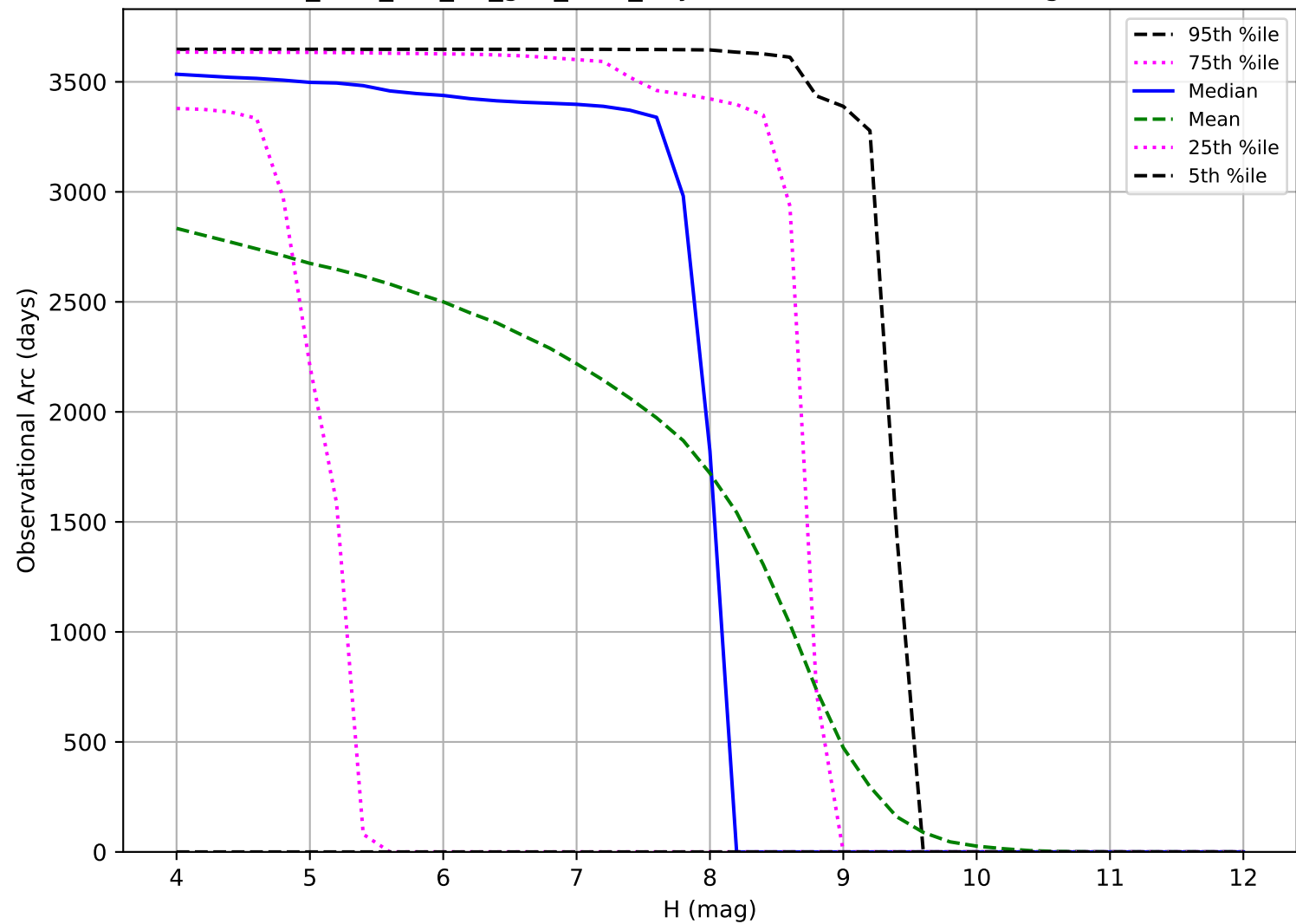
too_elab_r64_d2_griz_v3.4_10yrs: Observational Arc Length TNO
