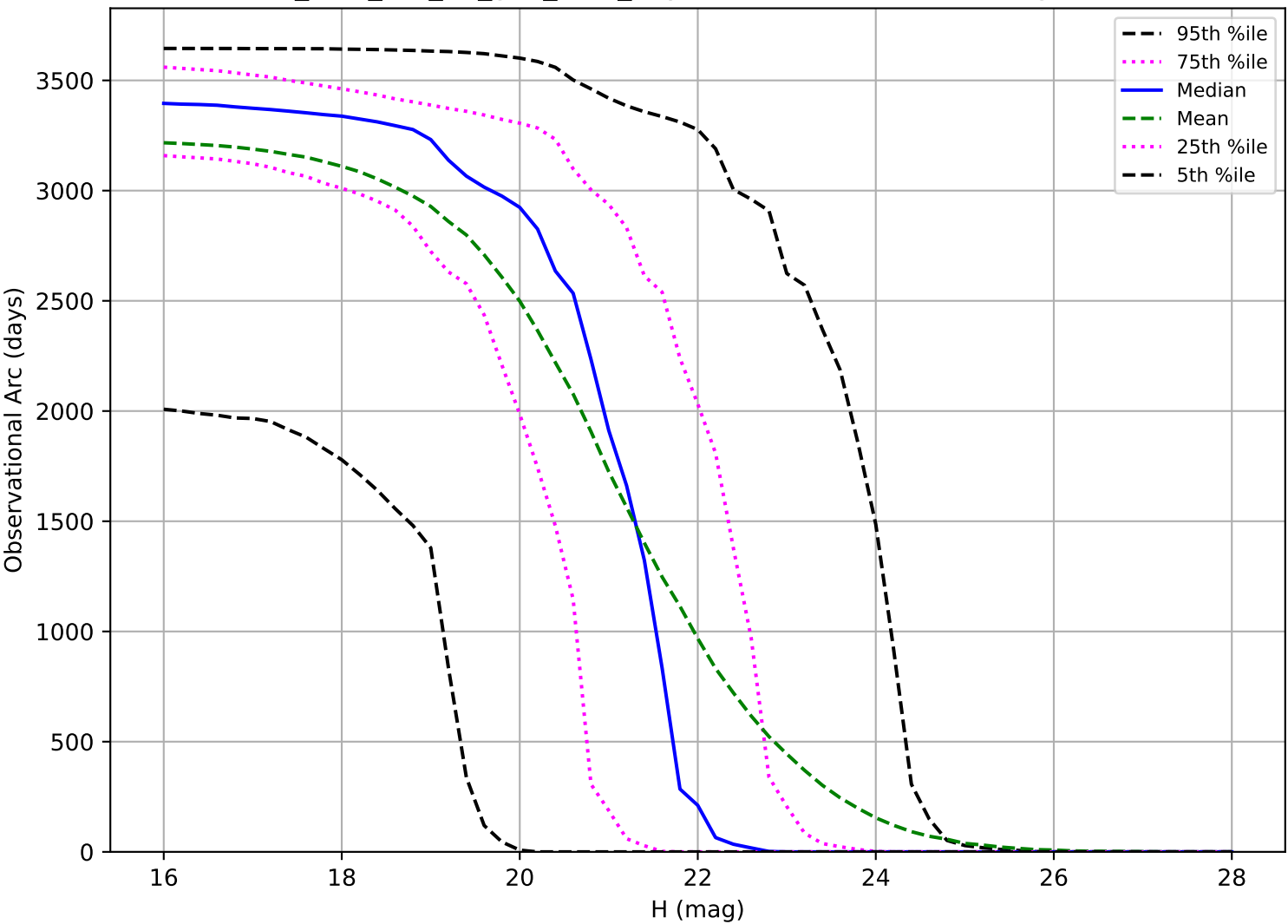
too_elab_r64_d2_griz_v3.4_10yrs: Observational Arc Length PHA
