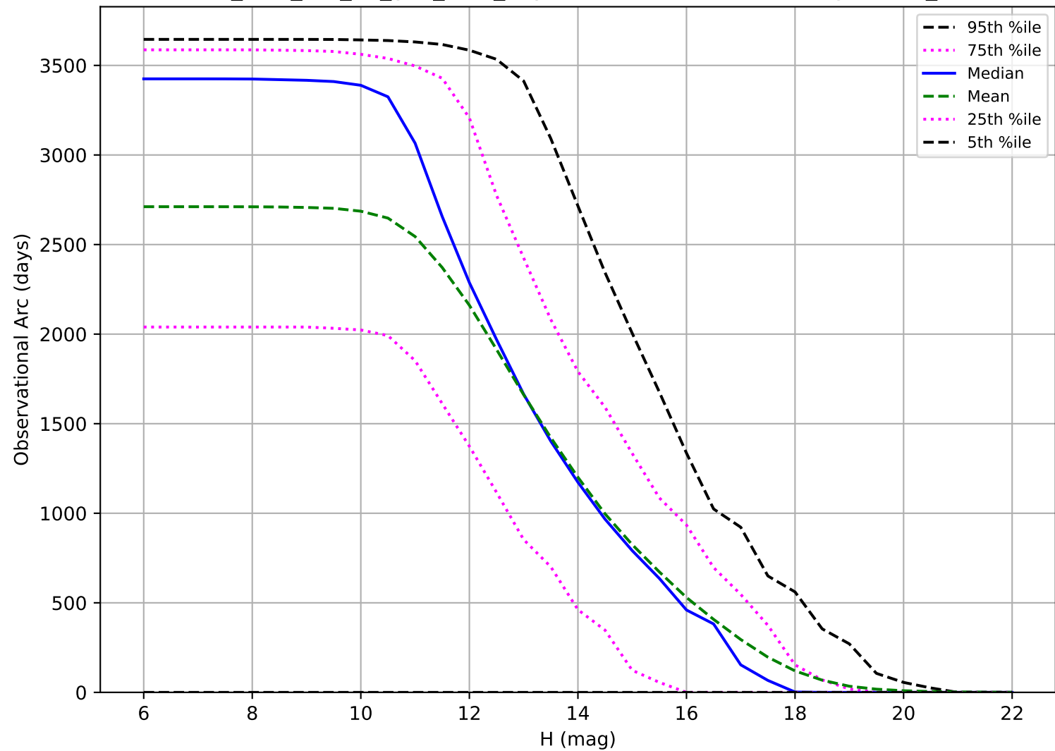
too_elab_r64_d2_griz_v3.4_10yrs: Observational Arc Length OCC_r5
