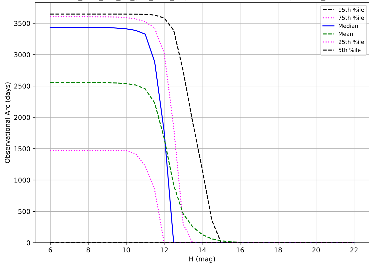
too_elab_r64_d2_griz_v3.4_10yrs: Observational Arc Length OCC_r20
