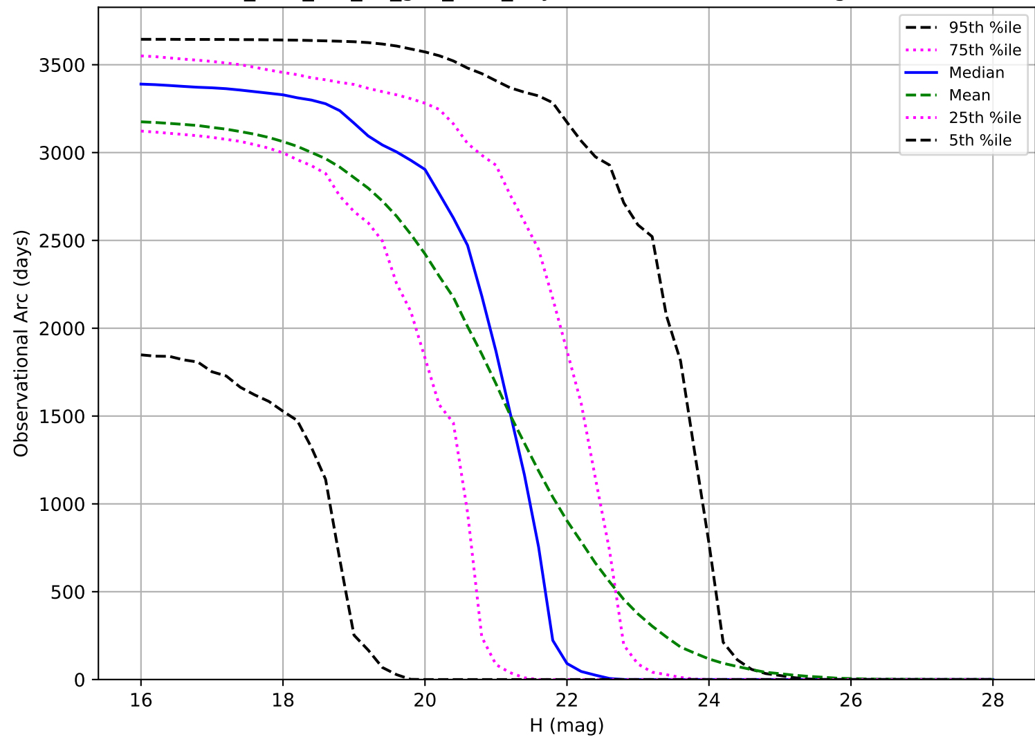
too_elab_r64_d2_griz_v3.4_10yrs: Observational Arc Length NEO
