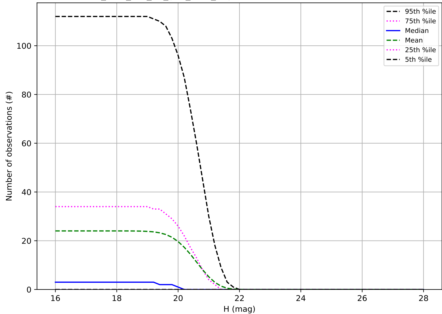
too_elab_r64_d2_griz_v3.4_10yrs: Number of observations Vatira
