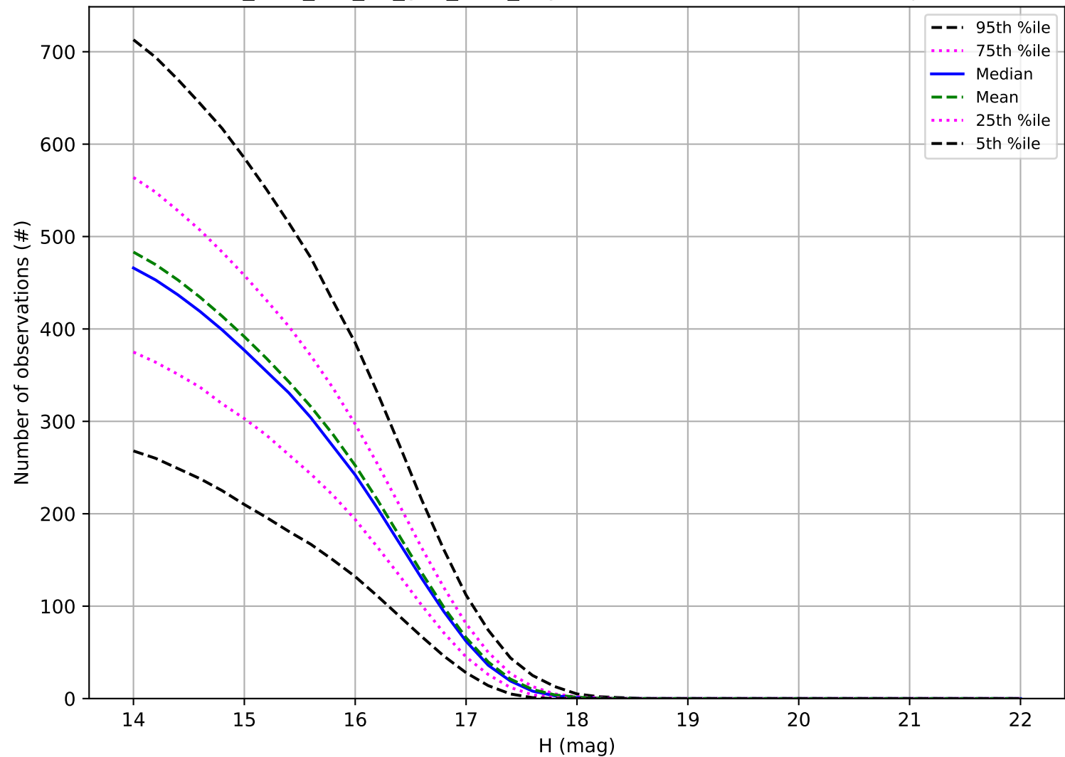
too_elab_r64_d2_griz_v3.4_10yrs: Number of observations Trojan
